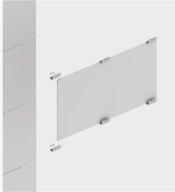
Middle clips
