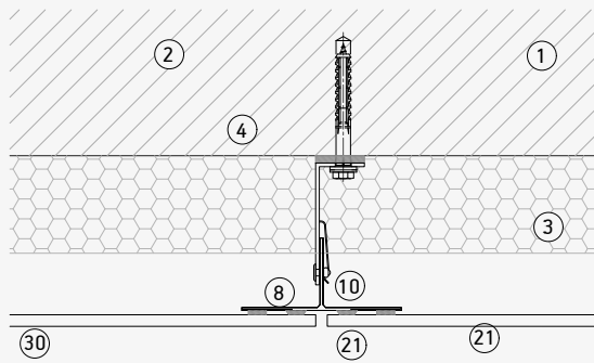
Vertical joint
