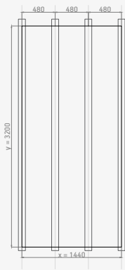
V2. Max. Design wind load: 11.0 kN/m 2
