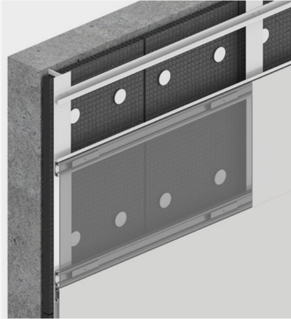
Profiles detail
