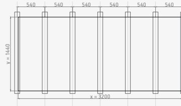
H3. Max. Design wind load: 2.0 kN/m 2
