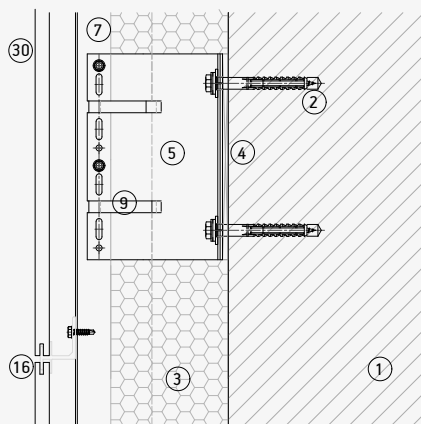
Horiozntal joint
