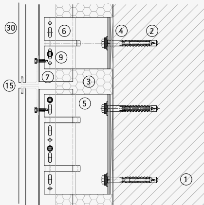
Joint between profiles
