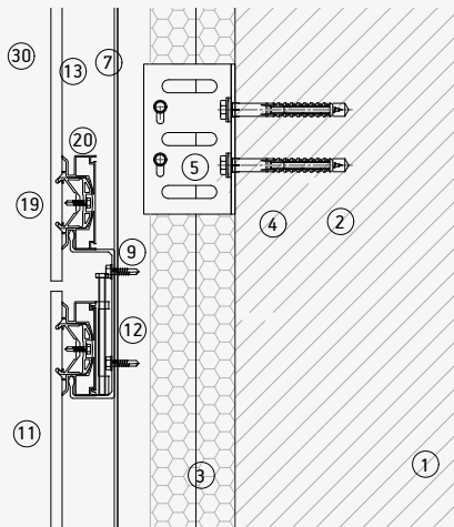
Horizontal joint
