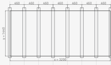
H5. Max. Design wind load: 2.5 kN/m 2
