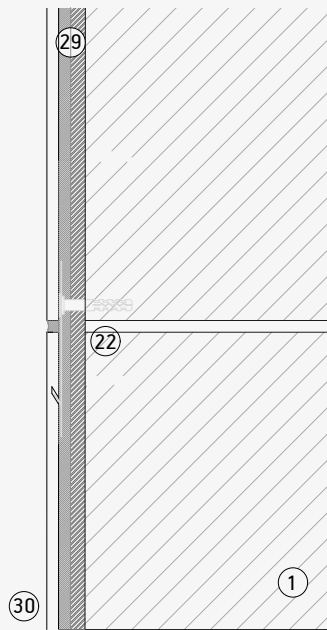
Horizontal profiles joint
