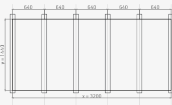
H4. Max. Design wind load: 5.0 kN/m 2
