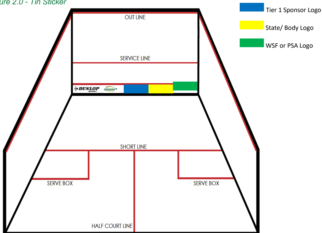
Figure 2.0 - Tin Sticker
